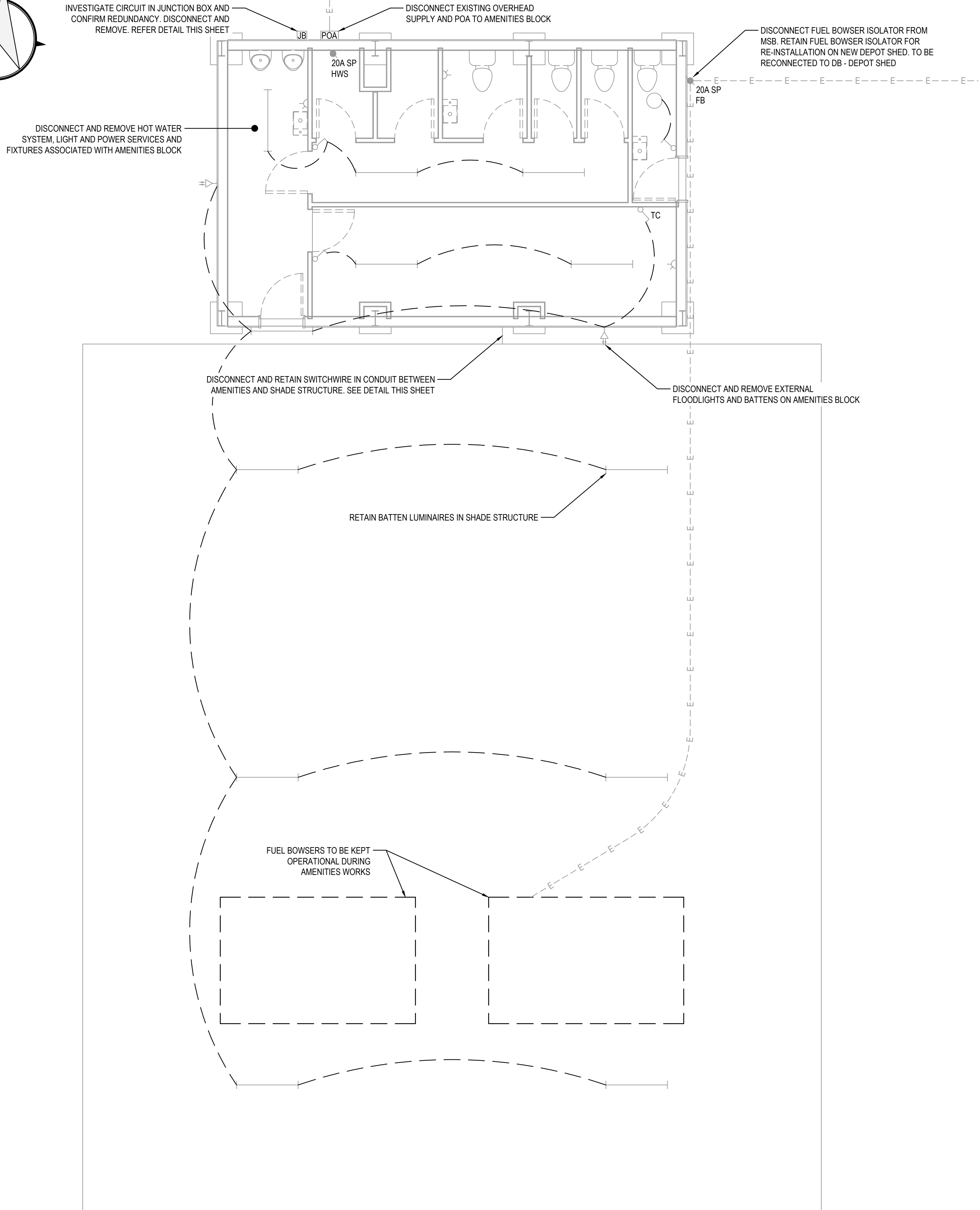
DEMOLITION PLAN 1:50
