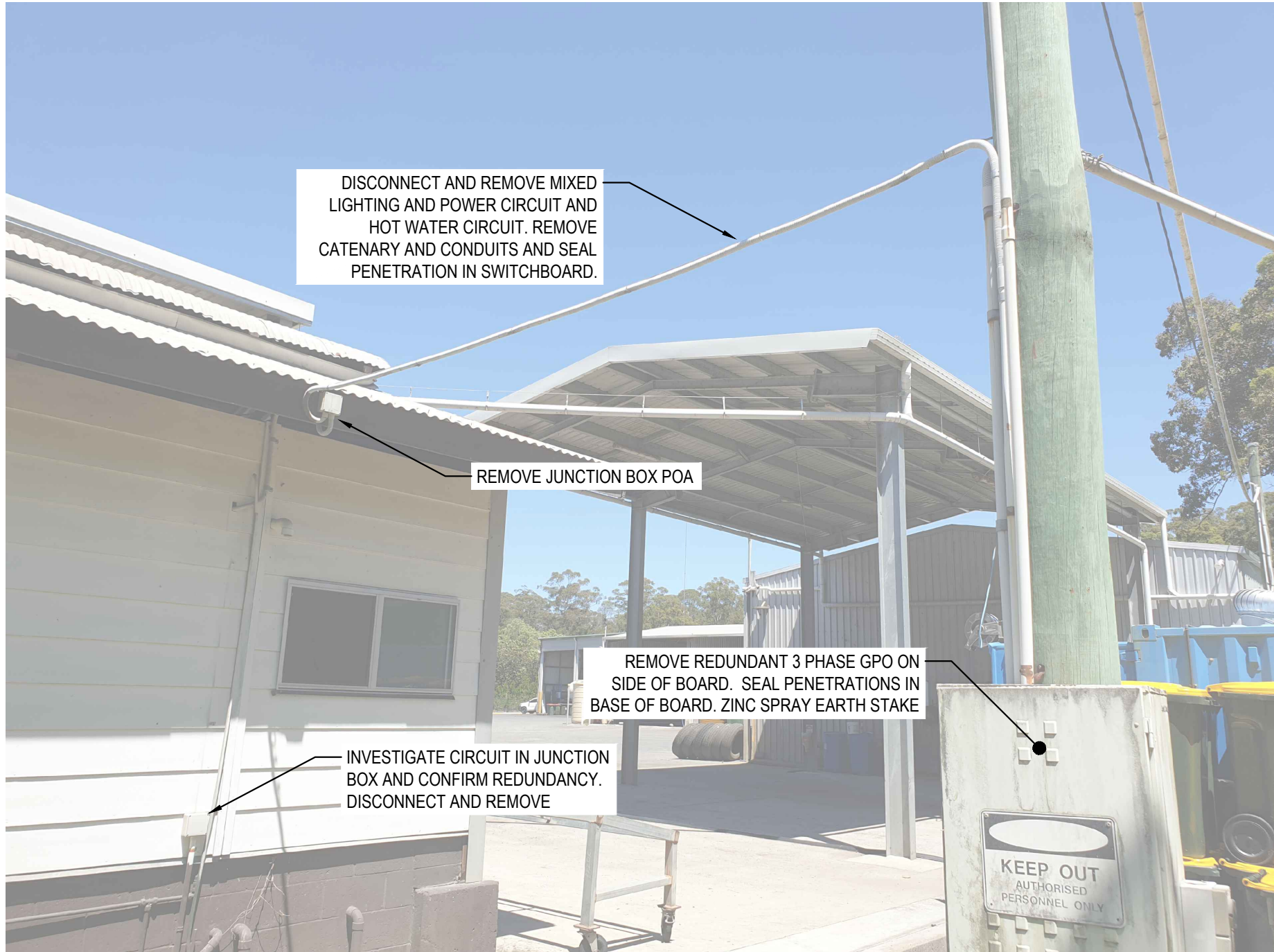
OVERHEAD ATTACHEMENT DETAIL 1:50
